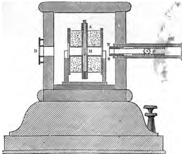
FIG. 98. Sectional Elevation.
